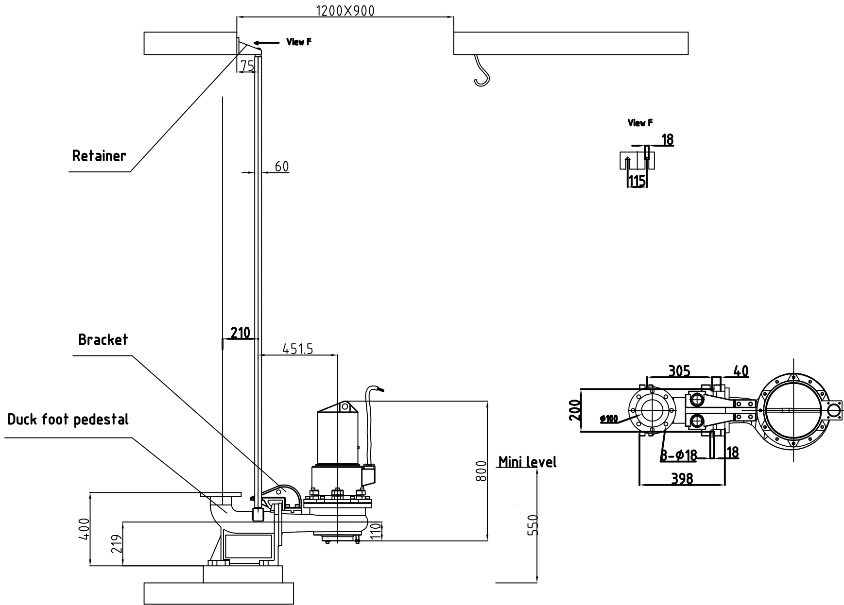
DN100 Duck foot installation system for SSP pump
