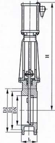
Main External And Connecting Dimensions(mm)
