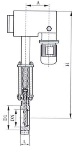
Main External And Connecting Dimensions(mm)
