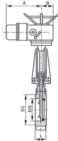
Main External And Connecting Dimensions(mm)
