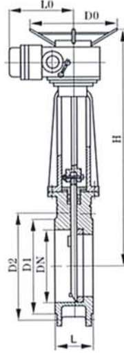
Main External And Connecting Dimensions(mm)
