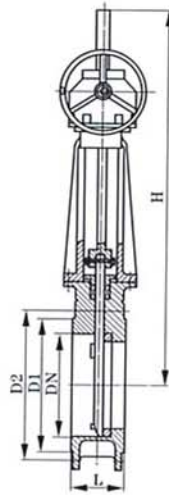
Main External And Connecting Dimensions(mm)
