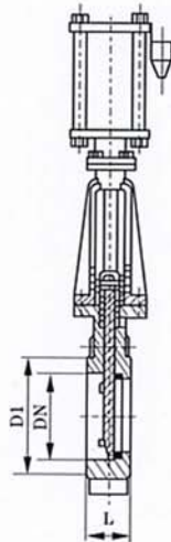
Main External And Connecting Dimensions(mm)
